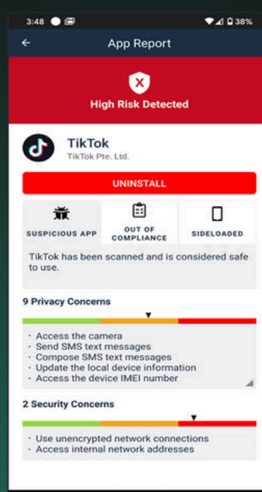
App Risk
