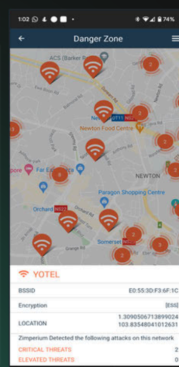
DangerZone
