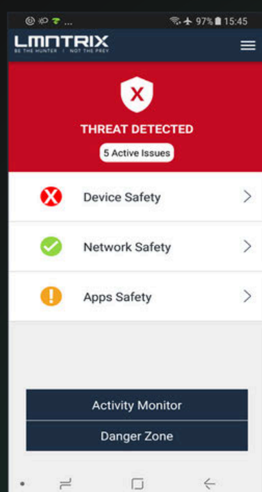
Device Risk
