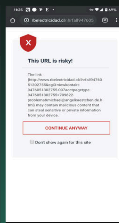
Phishing
